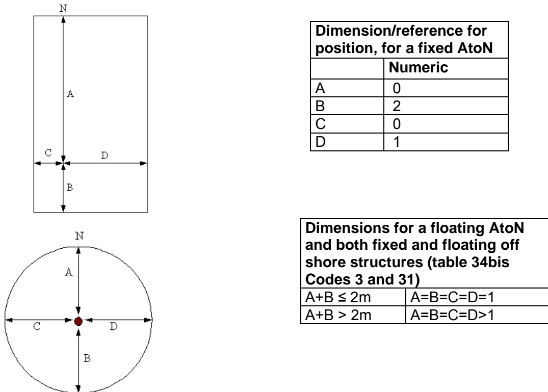
Figure 2 Dimension/reference for position AtoN field
