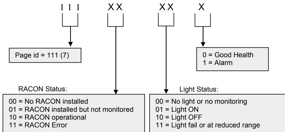
Figure 3 Recommended use of AtoN status bits
