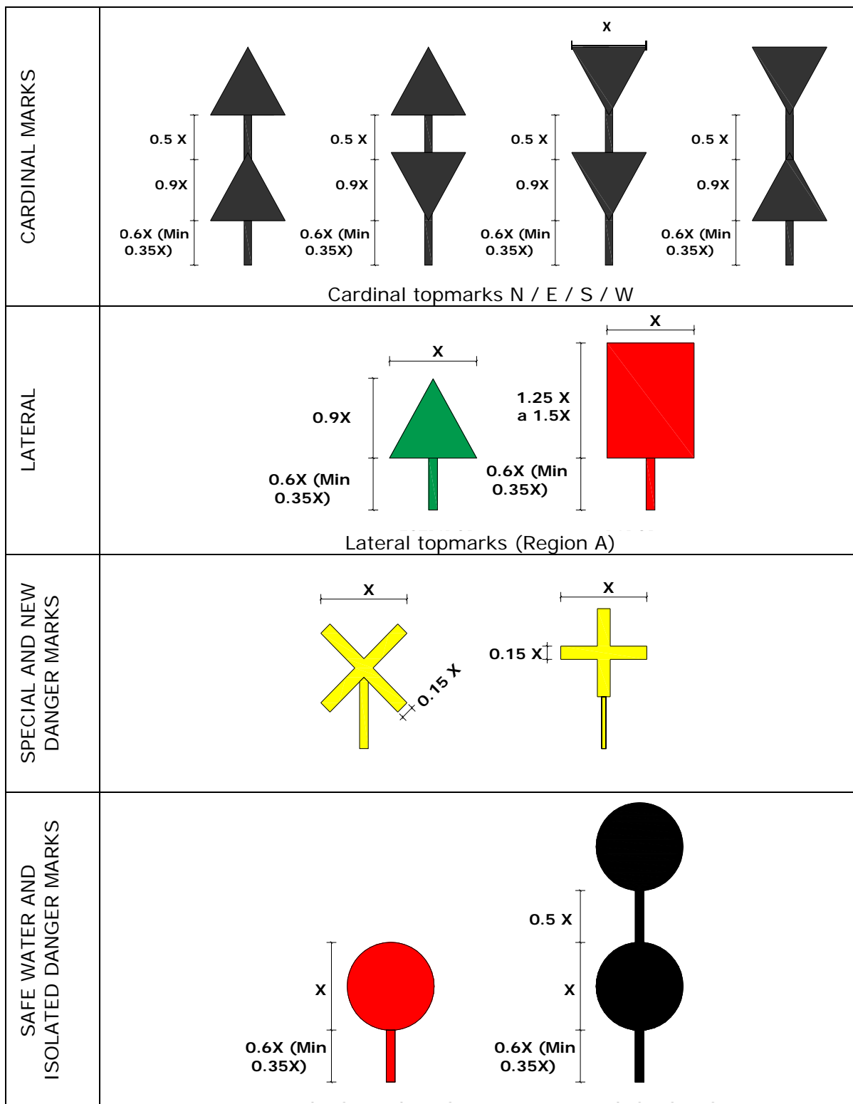
Figure 30 Topmark proportions
