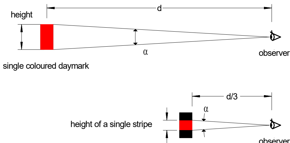
Figure 12 Single and multi coloured daymarks
